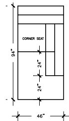
LOUNGER W: 46" D: 90" H: 30" SEAT D: 28"
