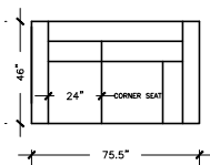
LOVE SEAT D W: 75.5" D: 46" H: 30" ARM H: 23" SEAT D: 28"
