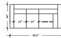
SOFA D W: 99.5" D: 46" H: 30" ARM H: 23" SEAT D: 28"
